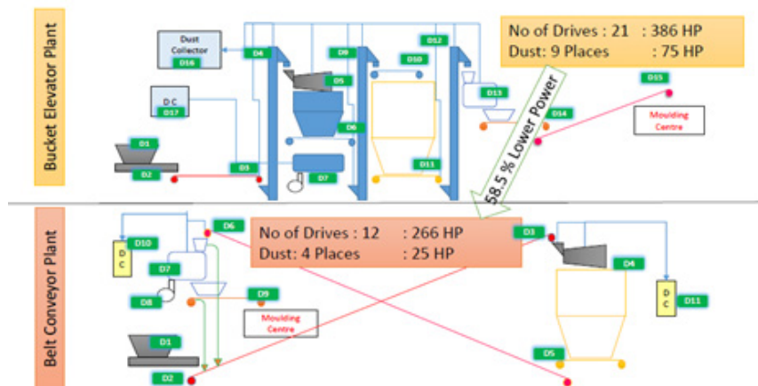
Figure 22: Comparison between bucket elevator plant and belt conveyor plant for sand handling
