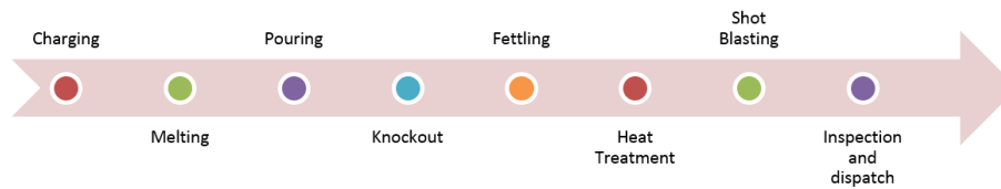
Figure 2: Process Flow
