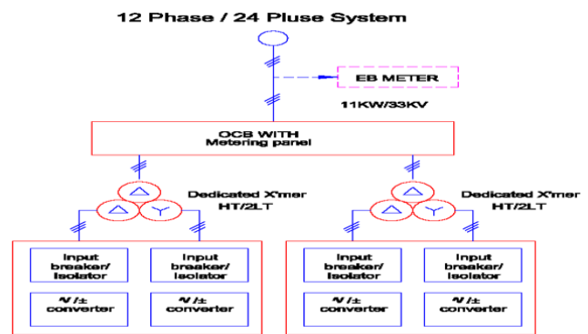
Figure 26: 12 Phase / 24 Pulse system
