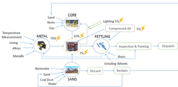
Figure 20: Energy share of critical processes in foundry industry
